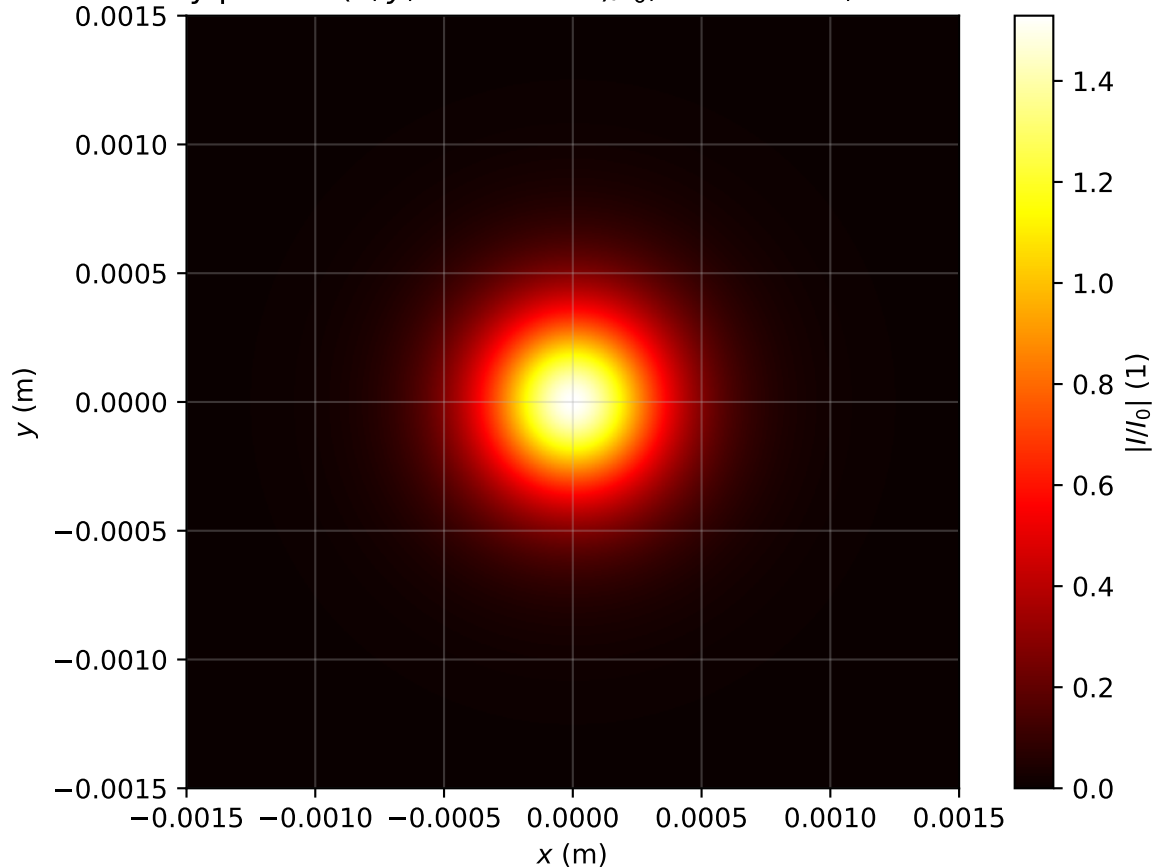
Intensity profile I(x, y, z = 3.264m)/I_0 , Pin=0.9Pcr, artificial time
